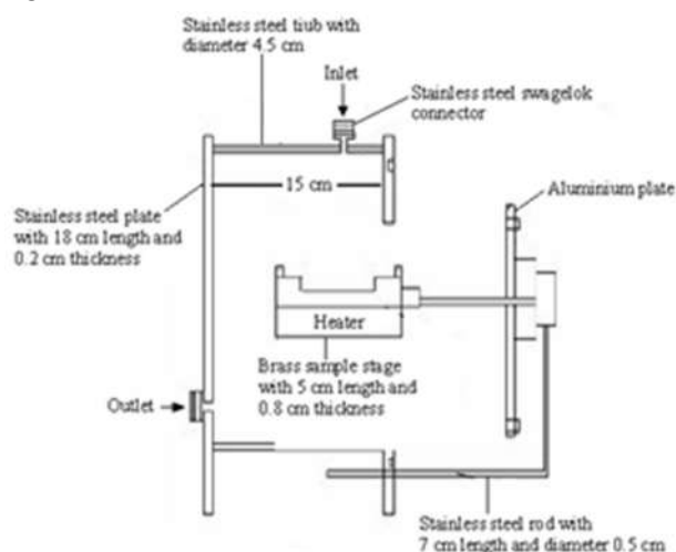
Rajah 1: Gas Test Chamber
